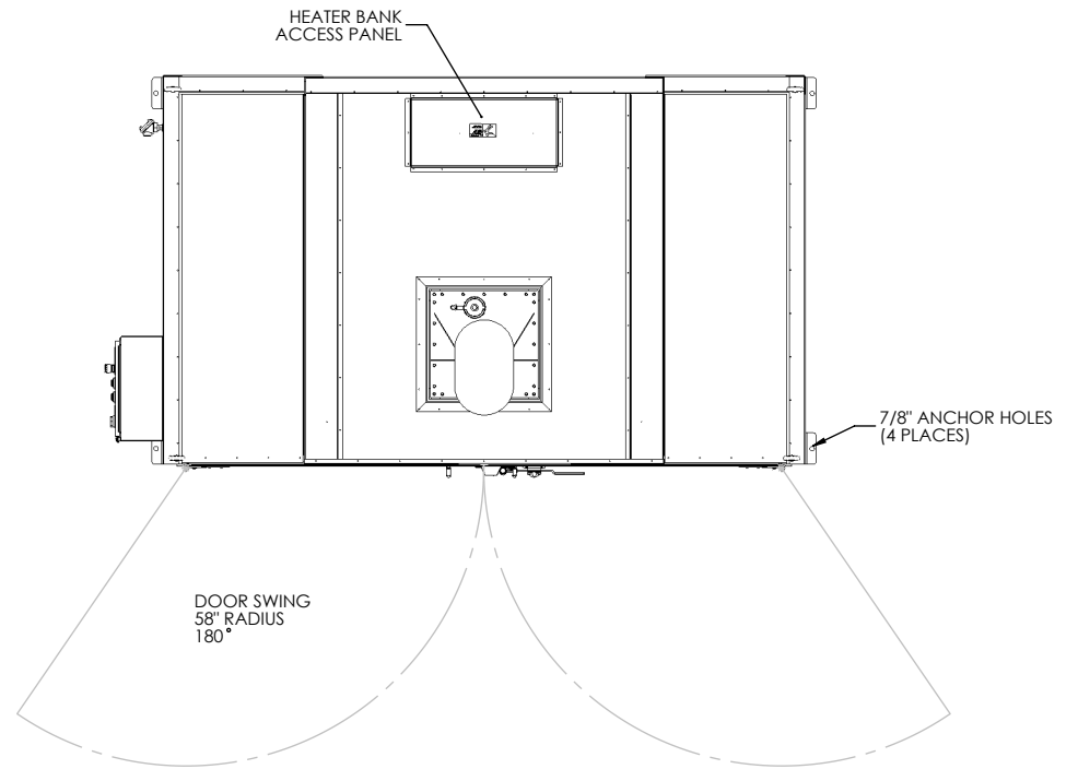
PLAN VIEW
