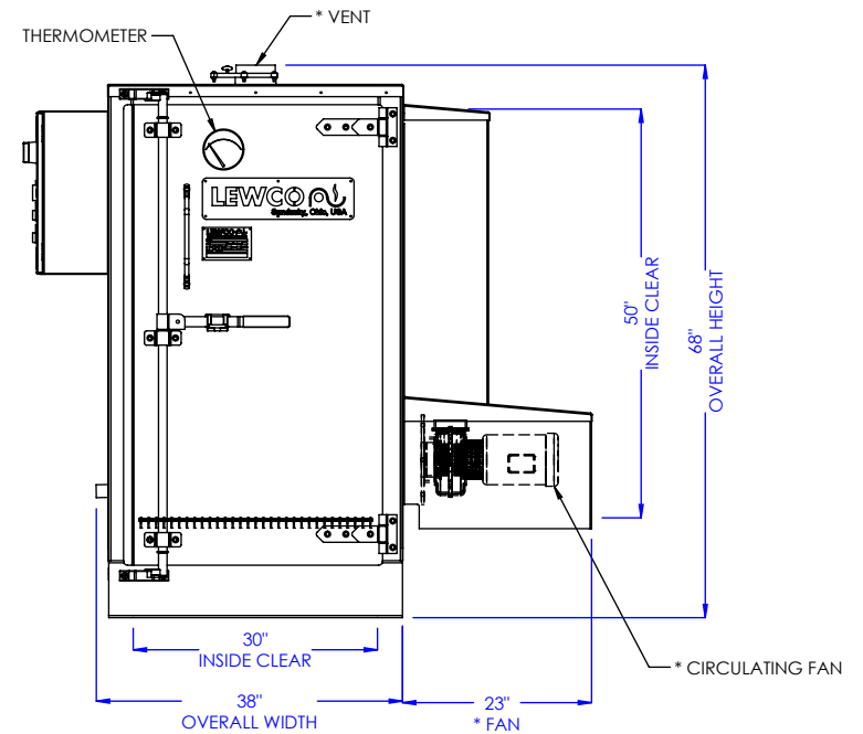
FRONT ELEVATION
