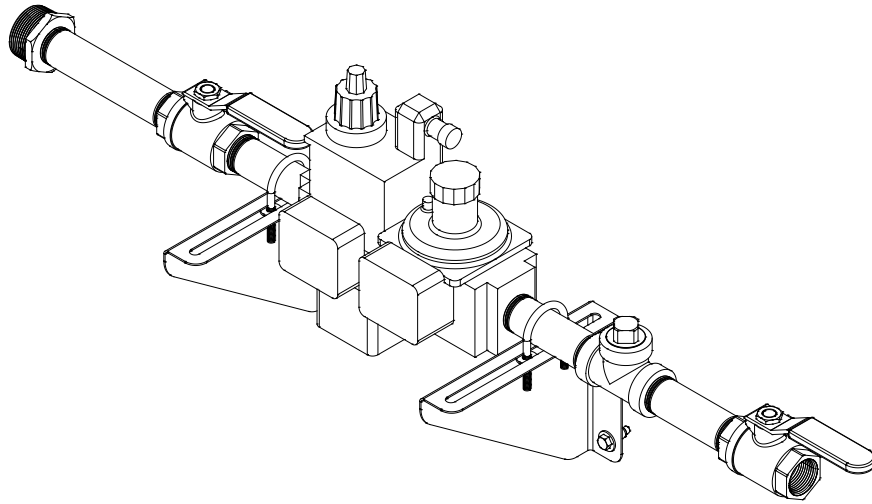
Typical LEWCO Gas Train
