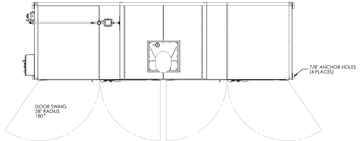
PLAN VIEW
