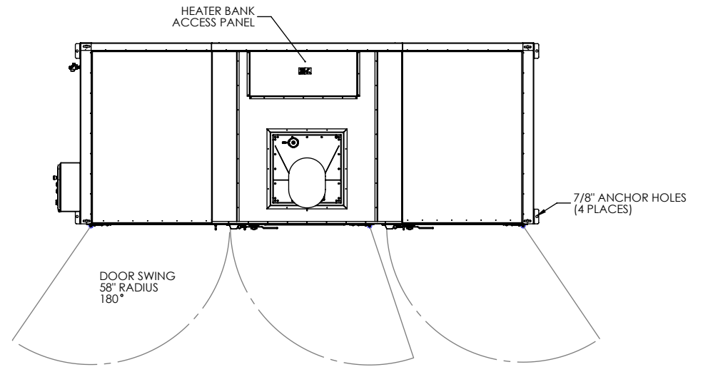
PLAN VIEW
