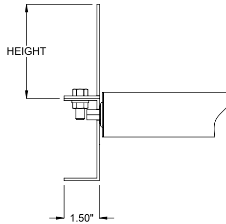
ANGLE GUARDRAIL
