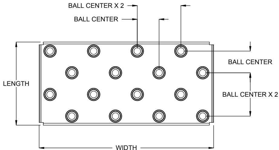
BALL TRANSFER TABLE STYLE D, STAGGERED BALL PATTERN
