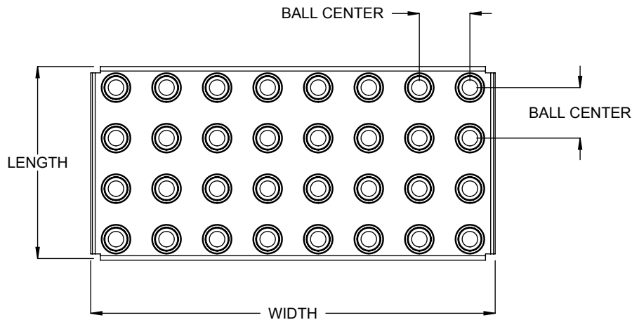
BALL TRANSFER TABLE STYLE D, STRAIGHT BALL PATTERN
